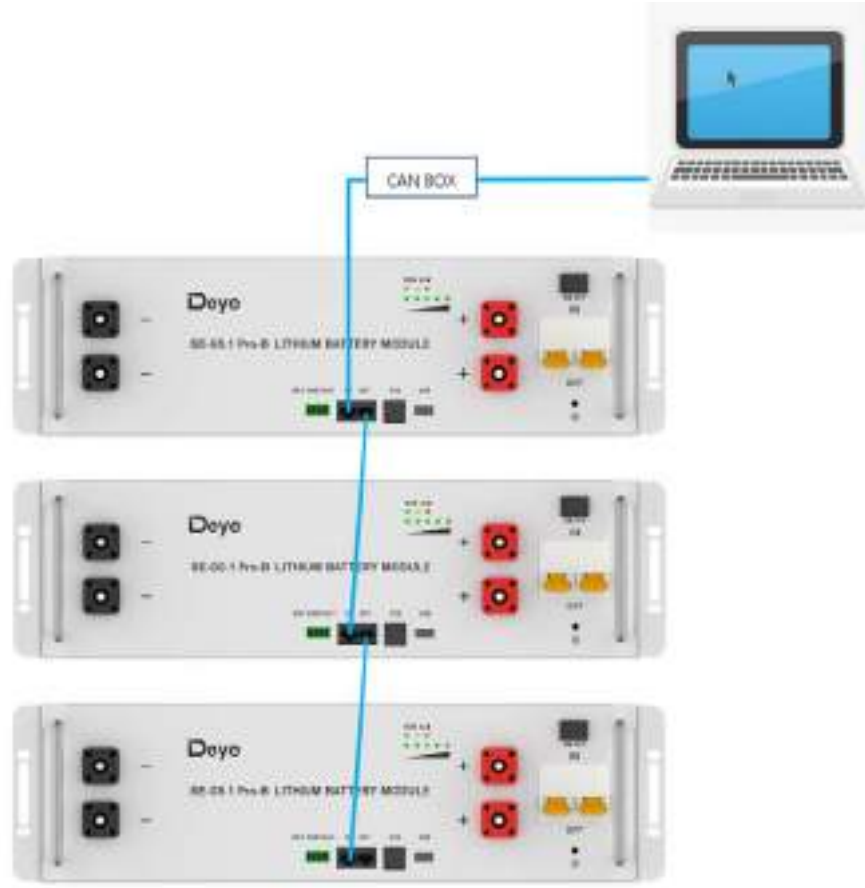
Figure 5-3: Communication Cable Connections between Battery and Computer
